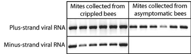
Fig. 4. Specific detection of plus- and minus-strand viral RNA in Varroa mites using tagged RT-PCR. Using a modified one-step RT-PCR protocol, V. destructor mites collected from freshly-hatched crippled and asymptomatic bees were individually analysed for the presence of plus- and minus-strand DWV RNA. Representative results are shown.
